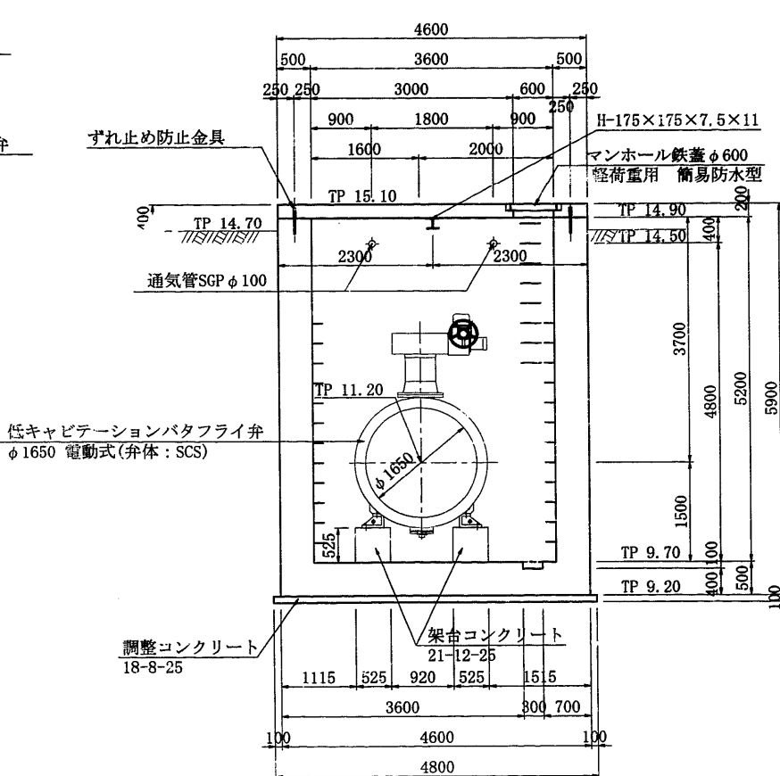
2-2 S=1:50
