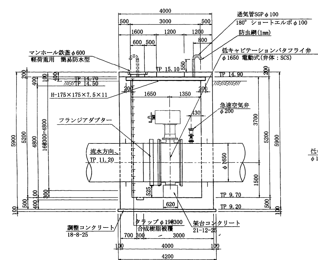
1-1 S=1:50
